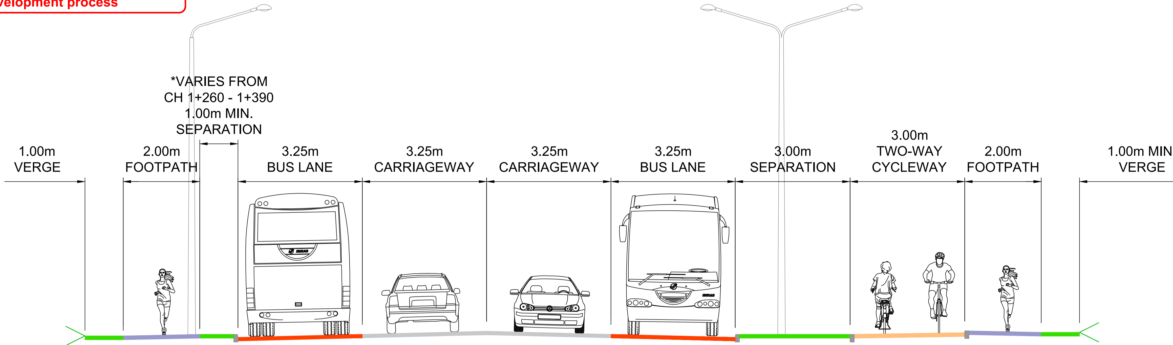
CROSS SECTION A
